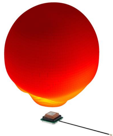
L5 3D RHCP Pattern @1176 MHz
