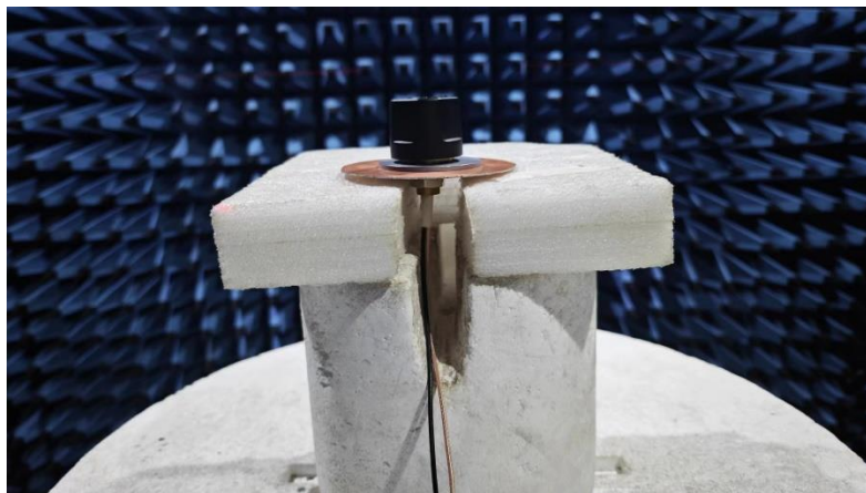
Radiation element is test on D120mm ground plane
