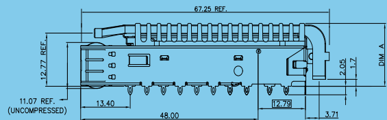
1xN Port Cage - Heat sink and Light Pipes
