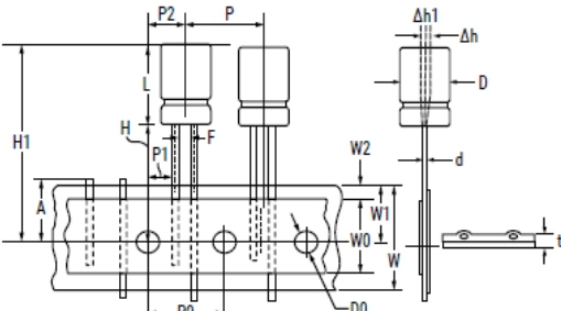
Fig. 4 (Diameter for Φ10) 10 mm EA
