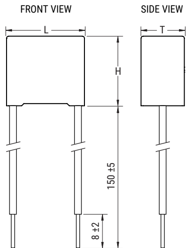
Insulated Flexible Leads 0.5 mm²
