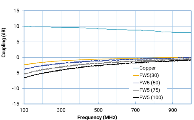
FW5 – Attenuation of Coupling Noise
