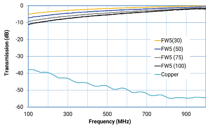
FW5 – Attenuation of Transmission Noise
