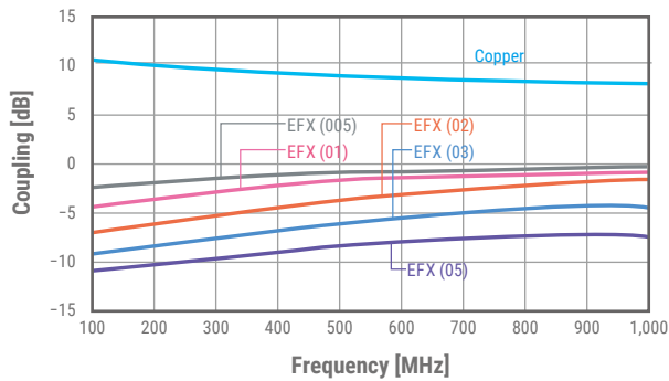
EFX – Attenuation of Coupling Noise
