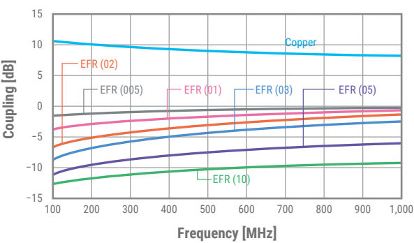
EFX – Attenuation of Coupling Noise
