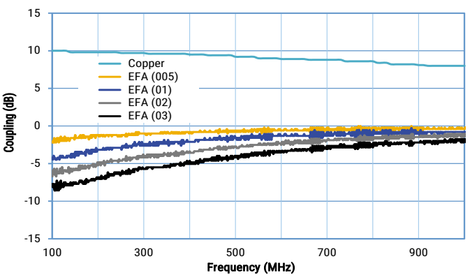
EFF4 - Attenuation of Coupling Noise
