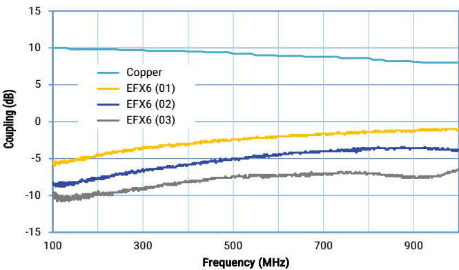
EFX6 – Attenuation of Coupling Noise
