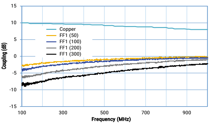
FF1 – Attenuation of Coupling Noise
