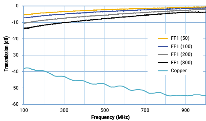
FF1 – Attenuation of Transmission Noise
