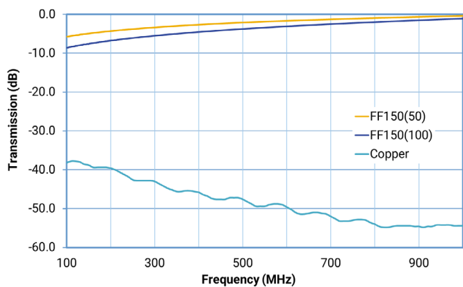
FF150 - Attenuation of Transmission Noise
