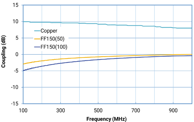
FF150 - Attenuation of Coupling Noise
