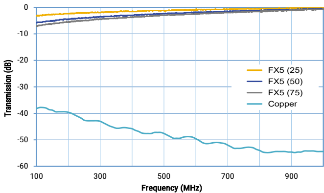
EFR – Attenuation of Transmission Noise
