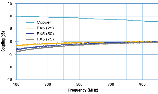
EFR – Attenuation of Coupling Noise
