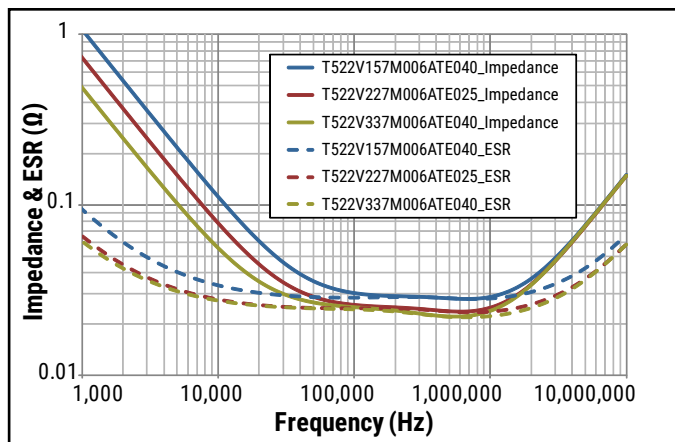
Impedance & ESR vs. Frequency
