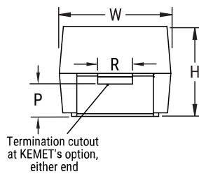
CATHODE (-) END VIEW
