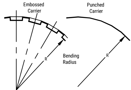
Figure 4 – Bending Radius
