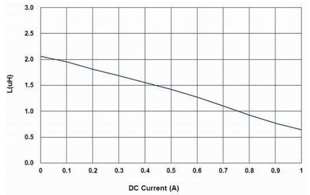
BKPE001608DZ2R2MA6
