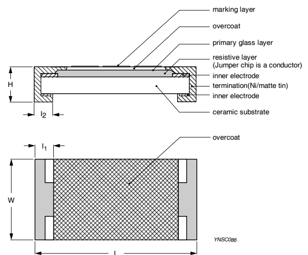
Fig. 4 Chip resistor outlines
