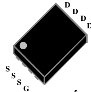
PMPAK ® 5x6
