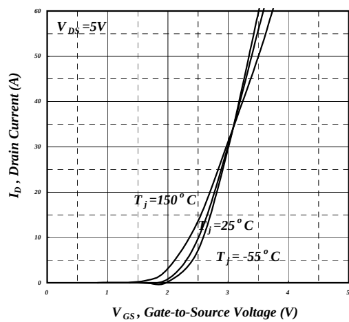
Fig 15. Transfer Characteristics
