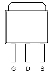
TO-251VS(JV)
