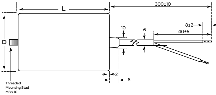
BiPolar Cable
