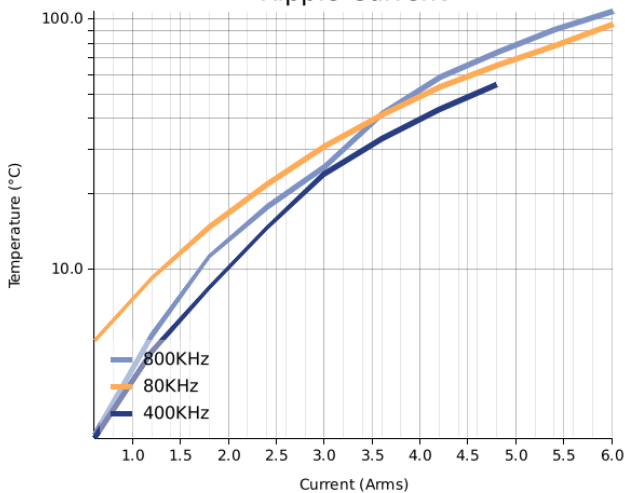
Ripple Current
